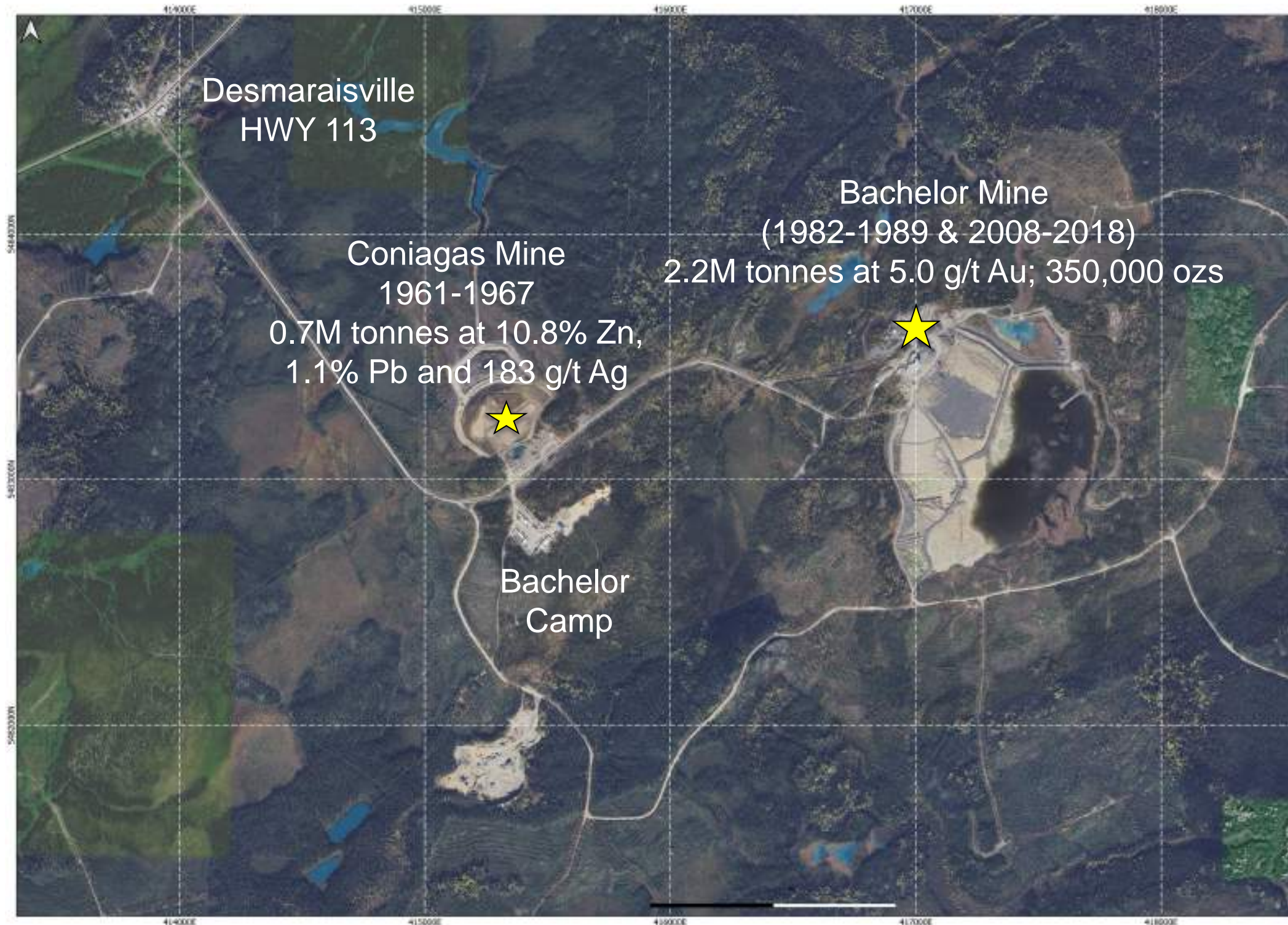
Plan View
